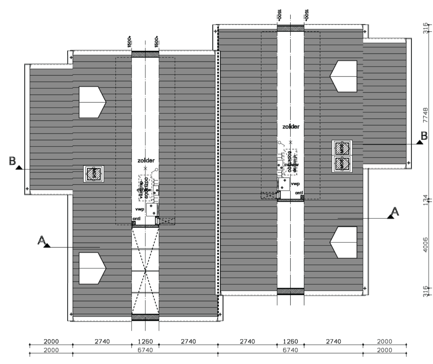
zolder
