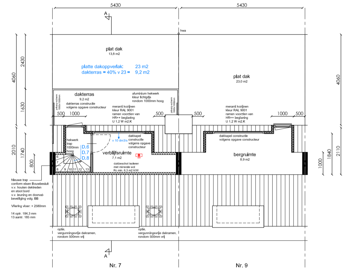
Zolderverdieping
