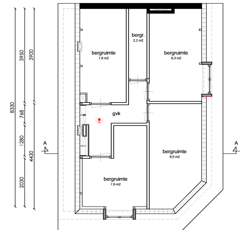
Zolderverdieping
