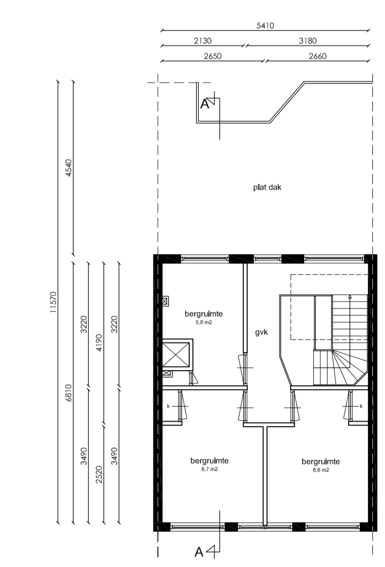
Zolderverdieping
