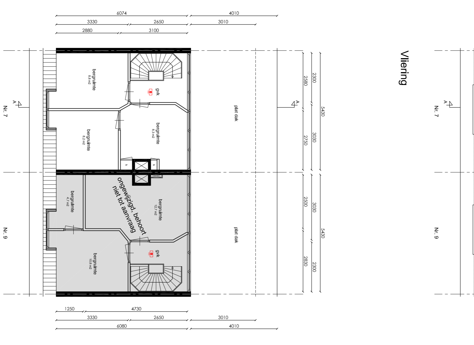
Zolderverdieping
