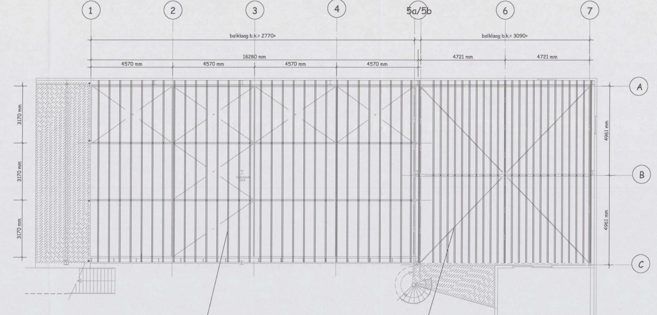
houten balklaag
