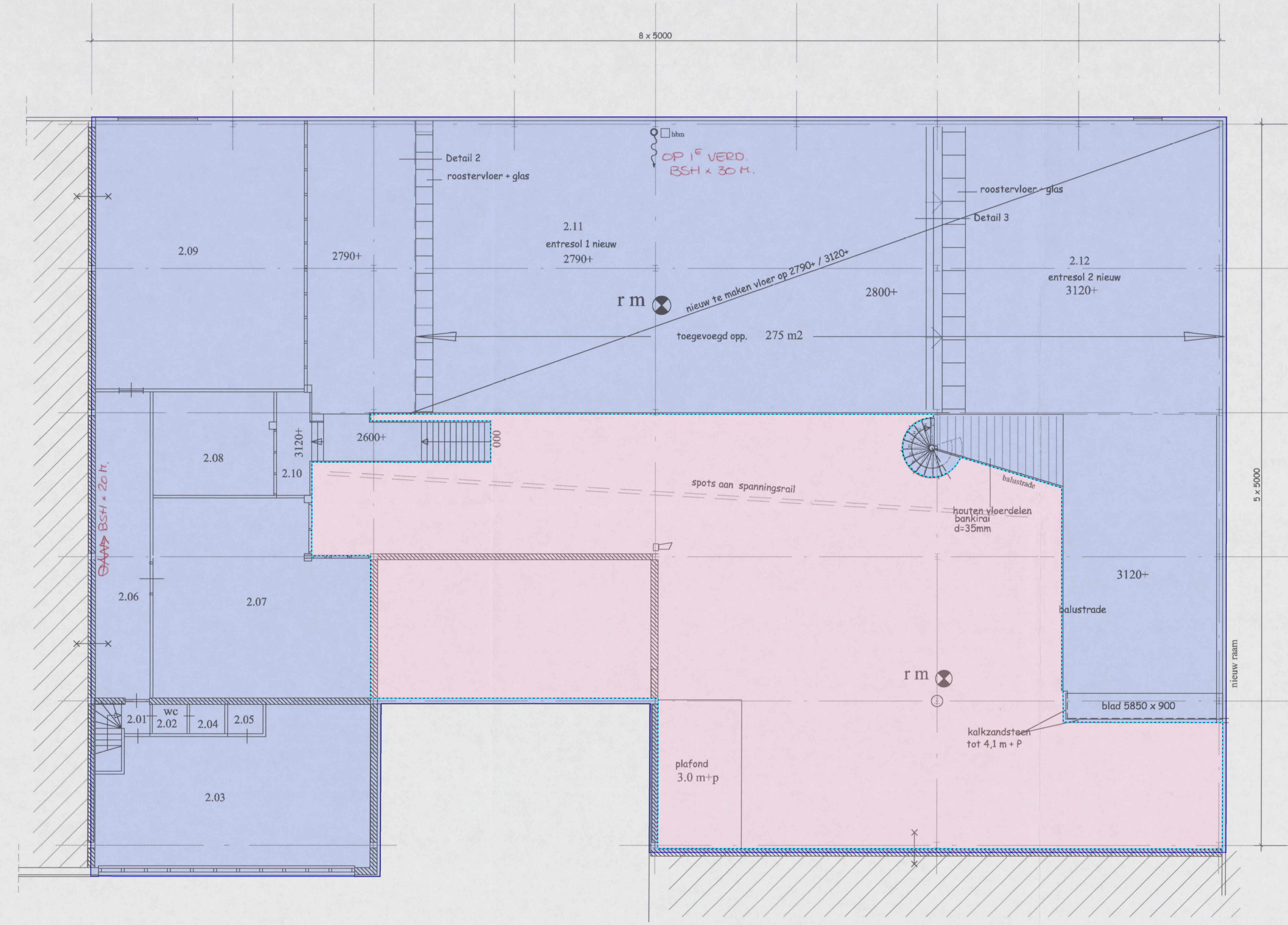
verdieping 2790+ / 3120+
