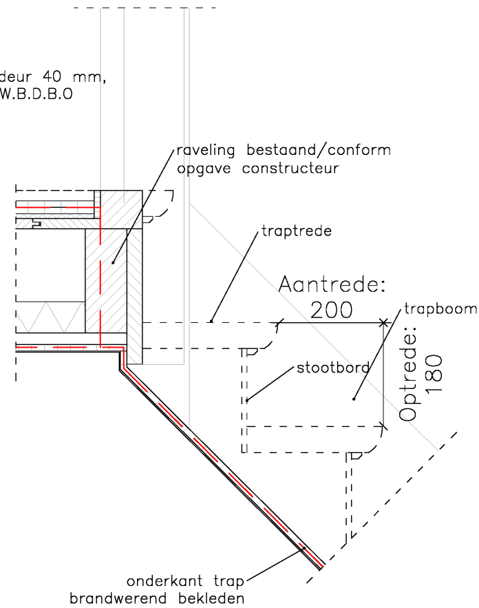
Detail P4 trap
