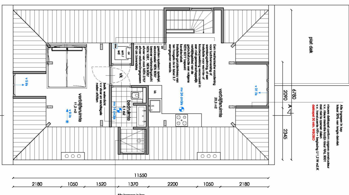
Zolderverdieping
