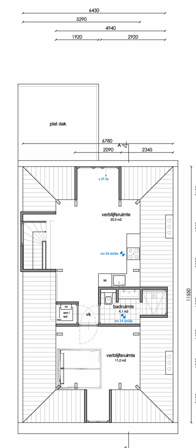
Zolderverdieping
