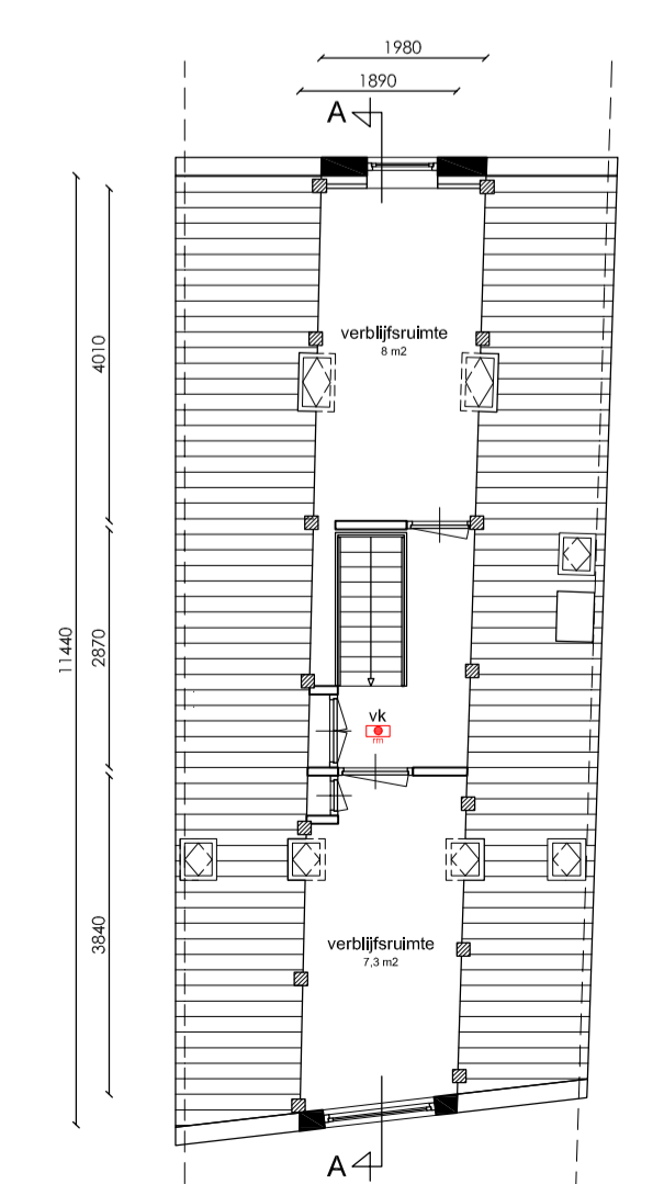
Zolderverdieping
