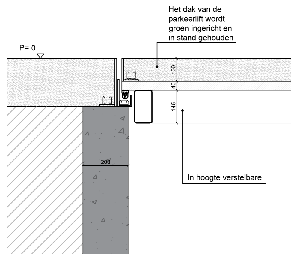
Detail A 1:10
