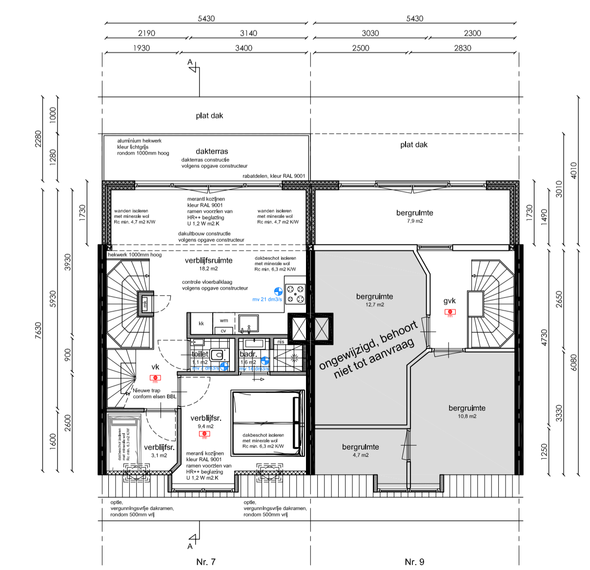
Zolderverdieping
