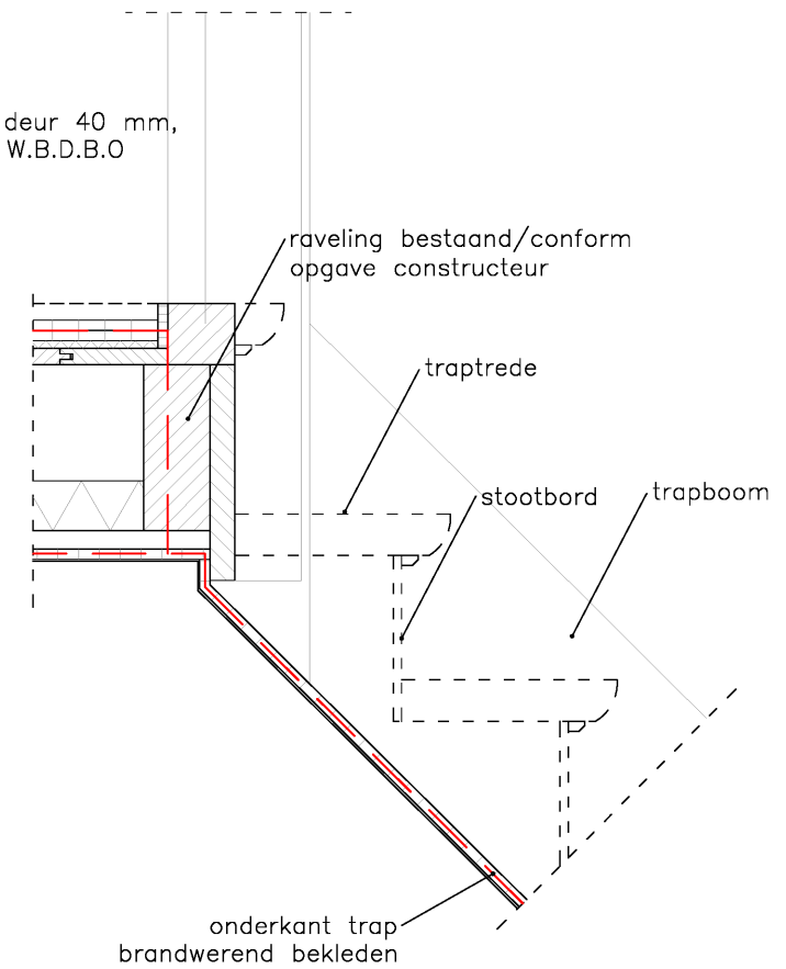
Detail P4 trap
