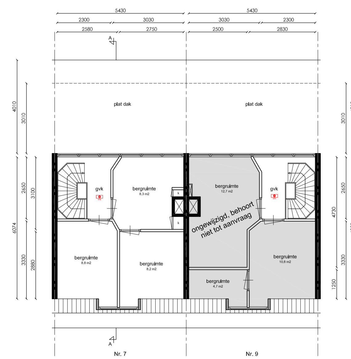
Zolderverdieping
