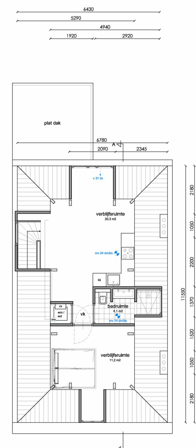
Zolderverdieping
