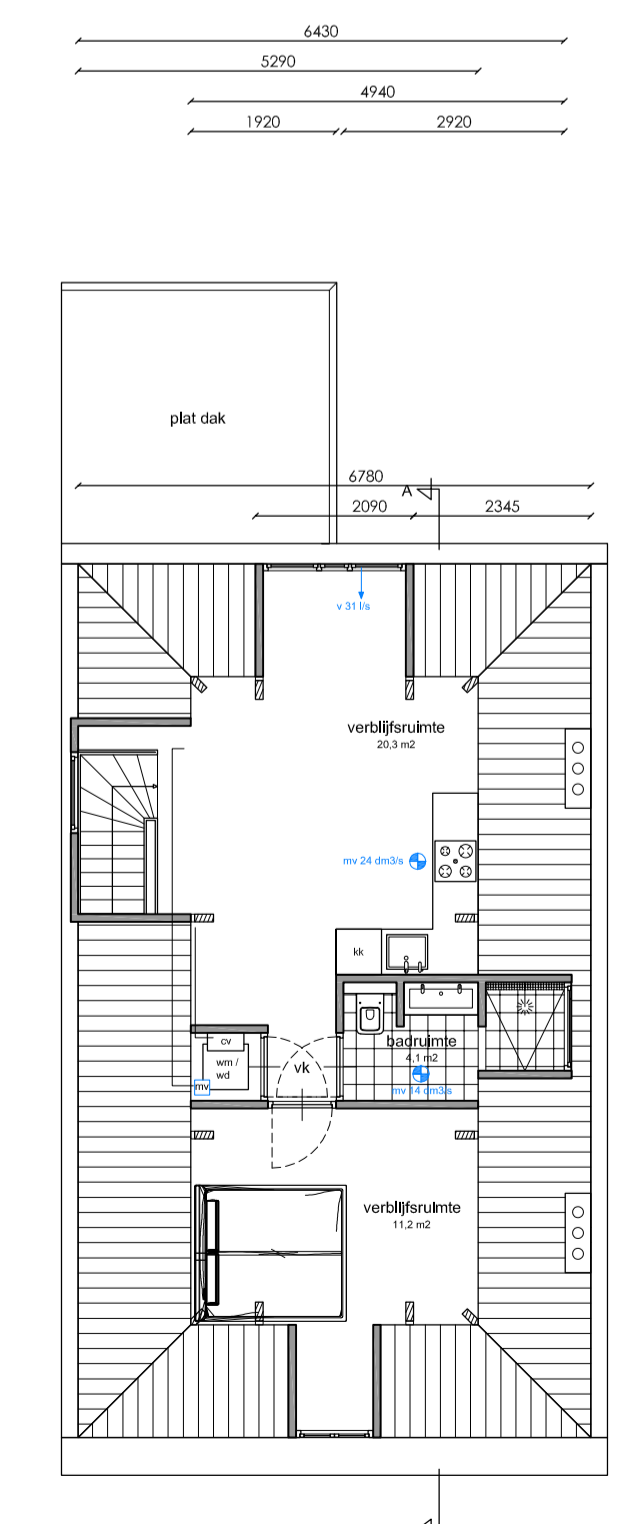
Zolderverdieping
