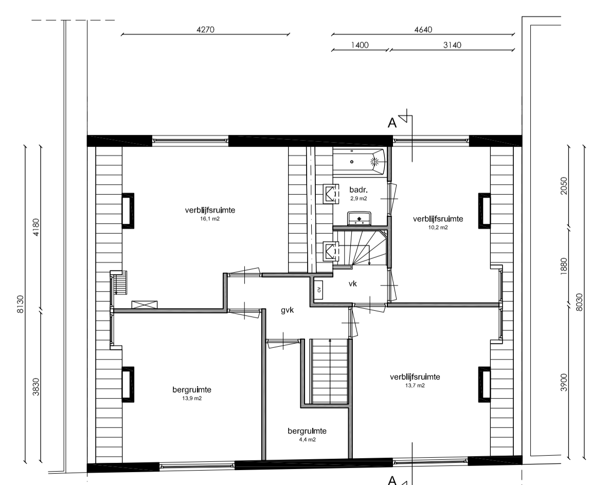
Zolderverdieping
