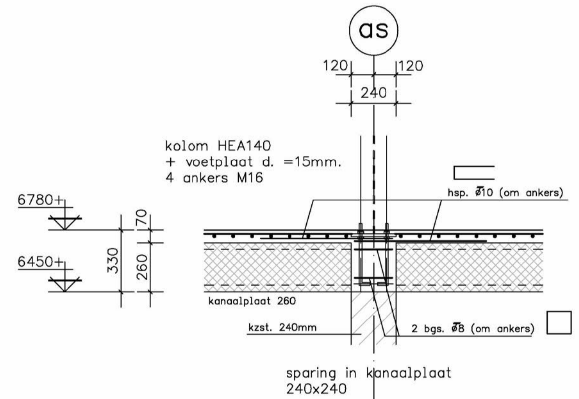
VERANKERING HEA 140.
