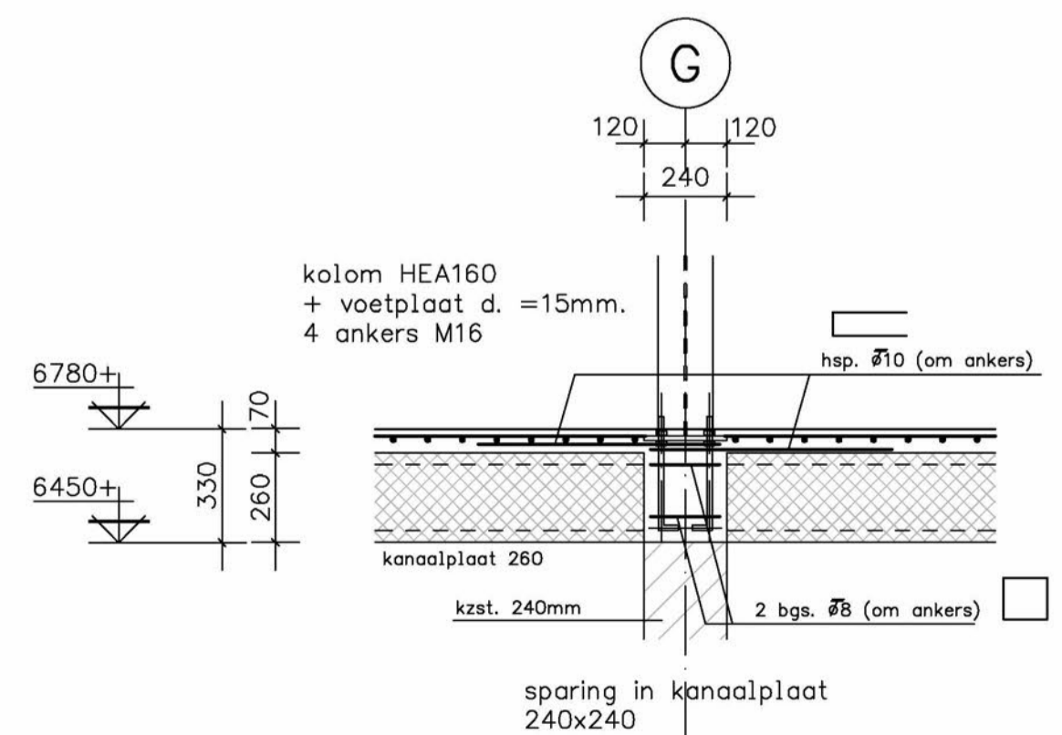
VERANKERING HEA 160.
