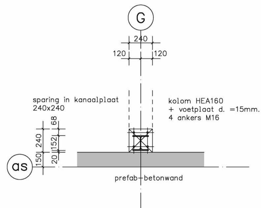
DETAIL 2
