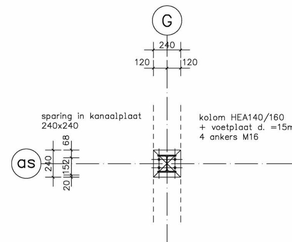
DETAIL 3
