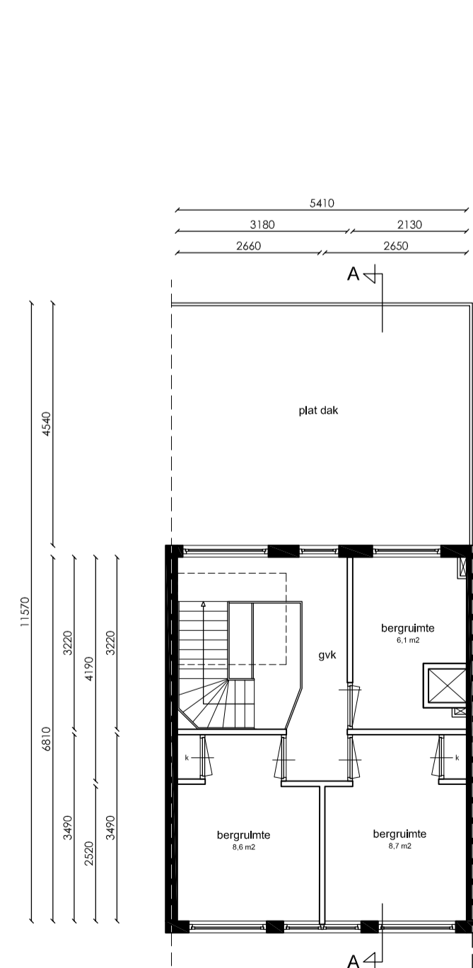
Zolderverdieping
