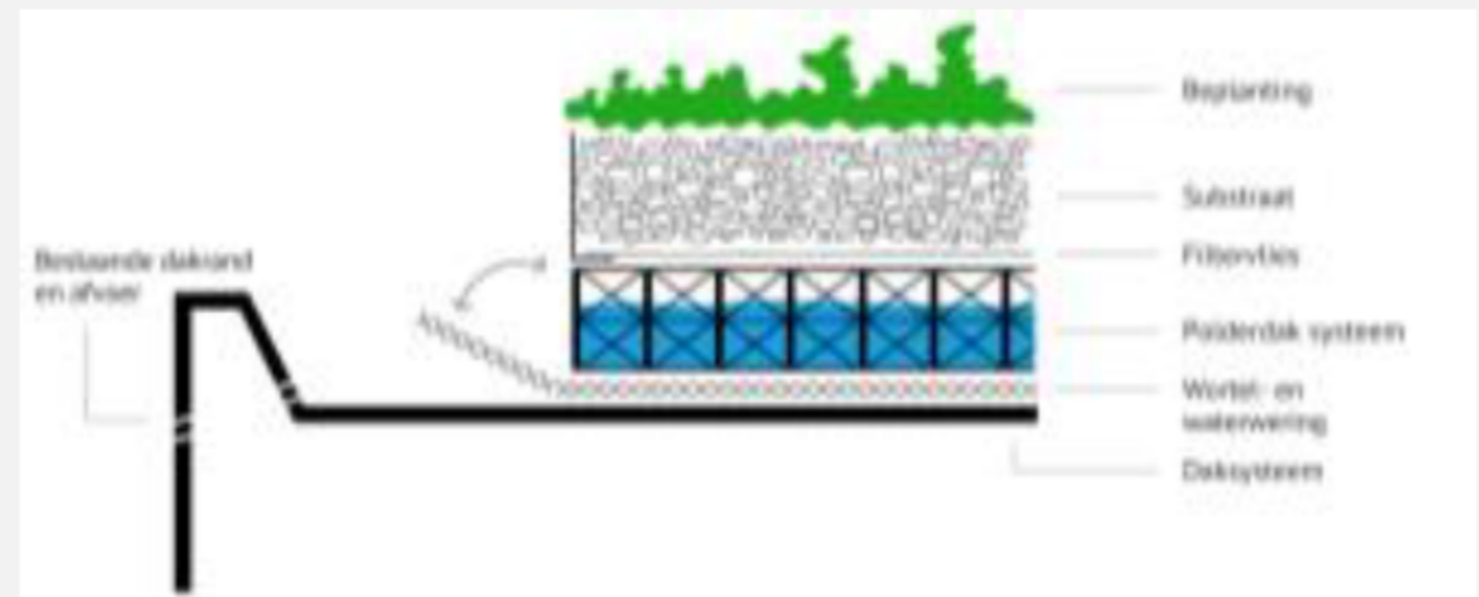
Polderdak ('Polderdak systeem' is drainage laag)
